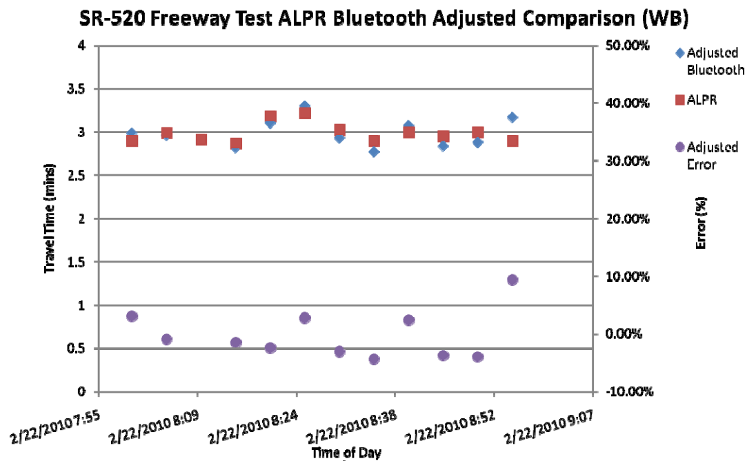
Figure 4-2: SR 520 freeway test
