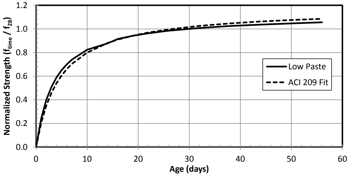
Figure 4.5: ACI 209 Specification Comparisons: DuPont (3/4-in.) Low-Paste
