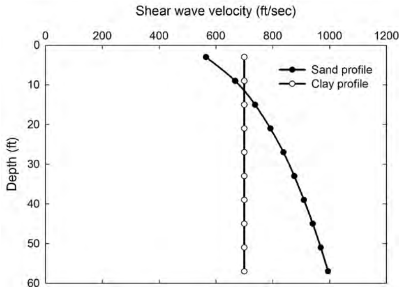
Figure 5.3 Shear wave velocity profiles for sand and clay soil profiles.
