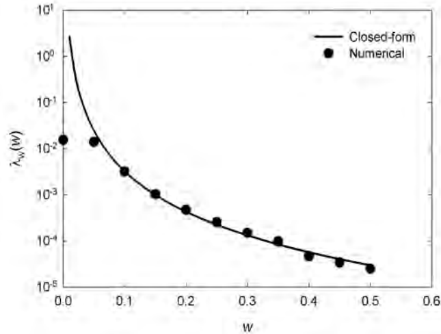
Figure 6.3 Comparison of closed-form and numerical solutions for deterministic base case vertical settlement problem and relatively coarse settlement increment.
