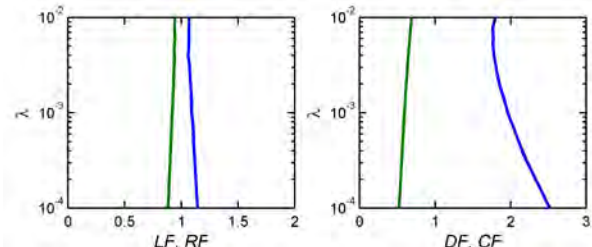
Figure 7.15 Load and resistance factors and demand and capacity factors for lateral loads and displacements at Seattle.
