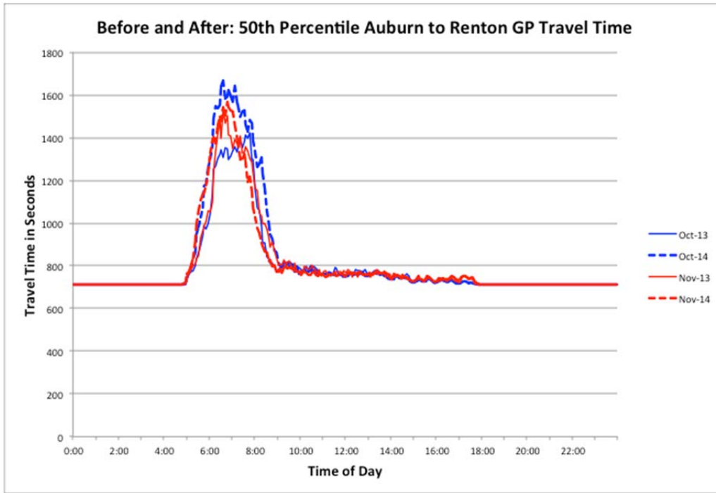
Figure 3-18: 50 th Percentile General Purpose Lane Travel Times, Auburn to Renton October and November Before and After Periods
