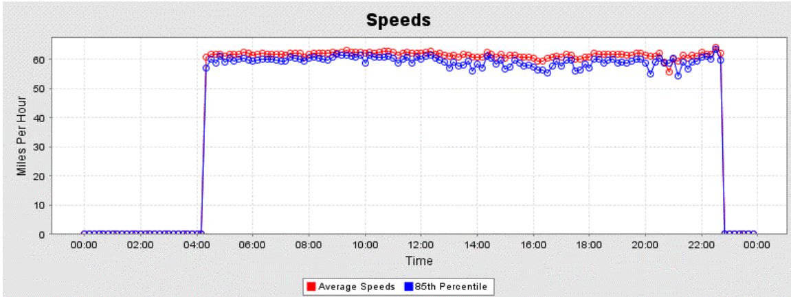
Figure 8: I-5 Northbound, Ridgefield–Ft. Lewis: Average Speed for the Mean and 85th Percentile (Slowest) Trip by Time of Day for All Weekdays March to June 2004
