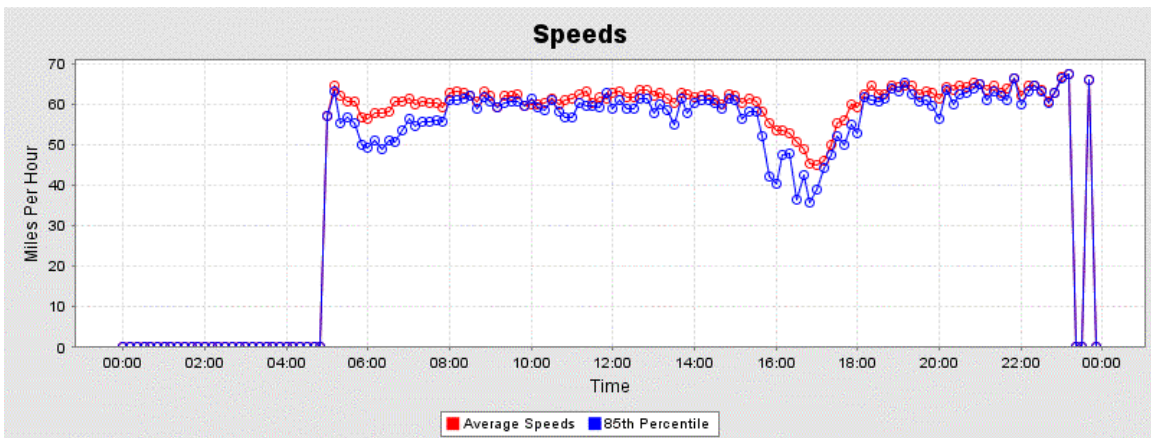
Figure 7: I-5 Northbound, Ft. Lewis to SeaTac: Average Speed for the Mean and 85th Percentile (Slowest) Trip by Time of Day for All Weekdays in May 2004
