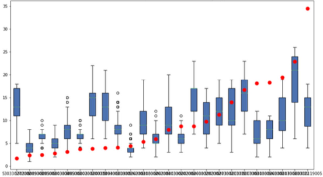
Distribution of XGB predictions over each block group
