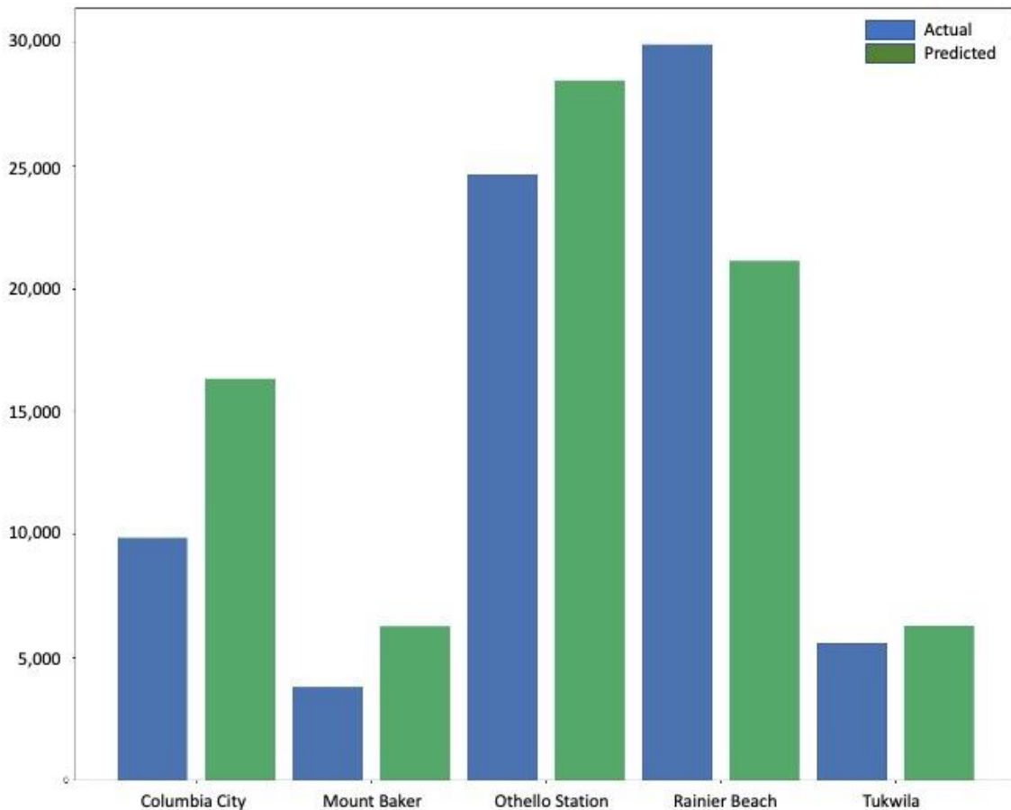
Figure 31: Link Station Summary of Model Prediction Accuracy
