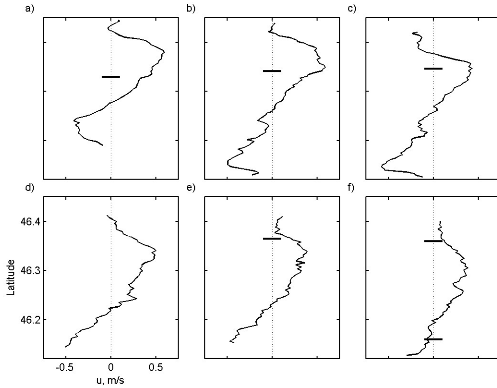
Figure 11: East velocity in the upper 5 m of the water column on Line B. The short thick line indicates the location of the tidal plume front determined from the surface salinity (see Figures 7, 8 and 9). Relative to the high tide before the greater ebb, the average time of each pass is a) 8.8, b) 11.6, c) 14.7, d) 19.8, e) 22.9, and f) 25.6 hours.
