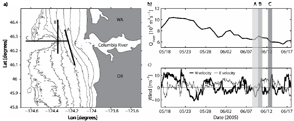
Figure 4: a) Locations for the three transects of interest during the June 2005 cruise. b) Columbia River discharge measured by the USGS at the Beaver Army Terminal, Quincy OR. (c) North and East wind velocity components from NOAA buoy 46026 near the mouth of the Columbia River. The shaded bars correspond to periods during which transects A, B and C (shown in a), were occupied.
