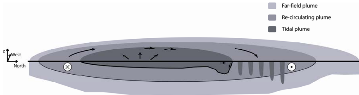
Figure 14: Cartoon showing the interaction between the three plume water masses from above and from the side under light wind conditions. The re-circulating plume flows in an anticyclonic direction within the far-field plume. The tidal plume initially propagates west, spreading north and south. As it approaches its westward extent, the tidal plume is deflected increasingly to the north.
