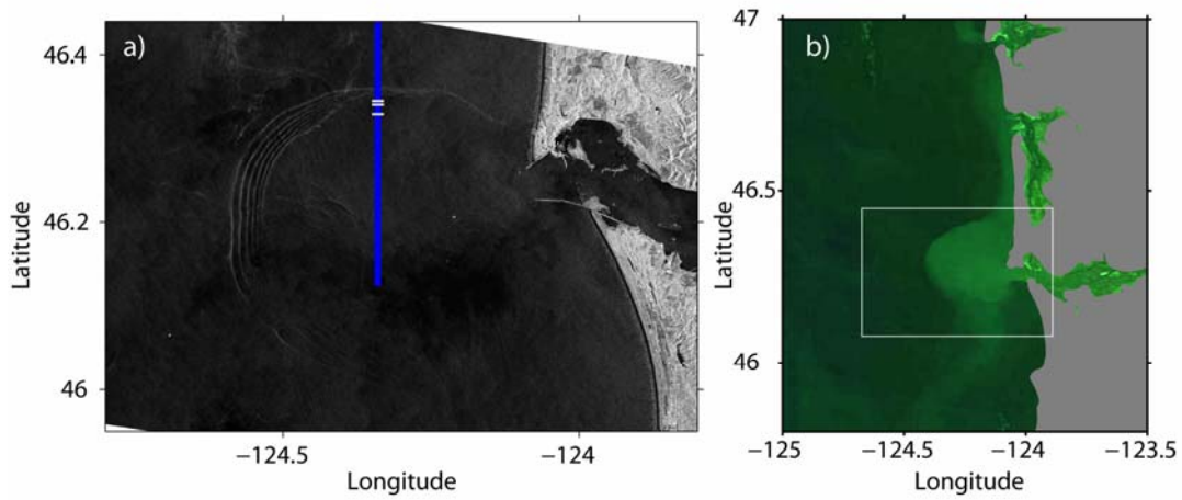
Figure 2: Remote imagery of the Columbia River plume. a) SAR image taken 10.5 hours after high tide on June 3, 2005. The semi-circular front and five solitons (outside the front) are evident as light colored lines in the image, which is sensitive to changes in surface roughness. The ship track for sampling on June 10, 2005 is shown in blue and the location of consecutive front crossings on that day is shown as white hatches on the transect line. b) True color image from the MODIS Terra sensor taken 5.5 hours after high tide on May 16, 2006. The image has been enhanced so that variability in the plume contrast is greater. The rectangle coincides with the region shown in a). Images are courtesy of Jiayi Pan, PSU (a) and Raphael Kudela, UCSC (b).
