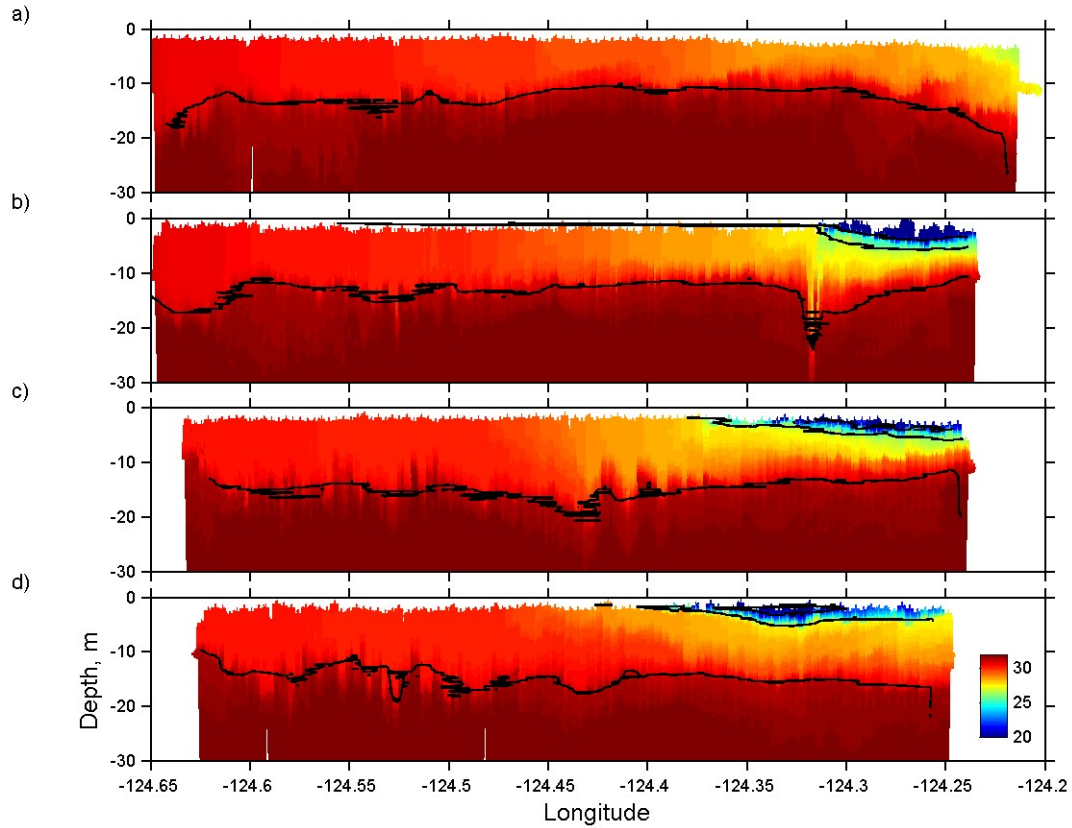
Figure 12: Salinity from the Triaxus towfish in the upper water column from Lines C2-C5, 2.4 – 11.1 hours after high tide, respectively, on June 13-14, 2005. The black lines are 21, 26 and 32 salinity isohalines, which approximately delineate the tidal, re-circulating and far-field plume water masses. a) - d) correspond to panels b) – e) in Figure 10, where the tidal phase is indicated.
