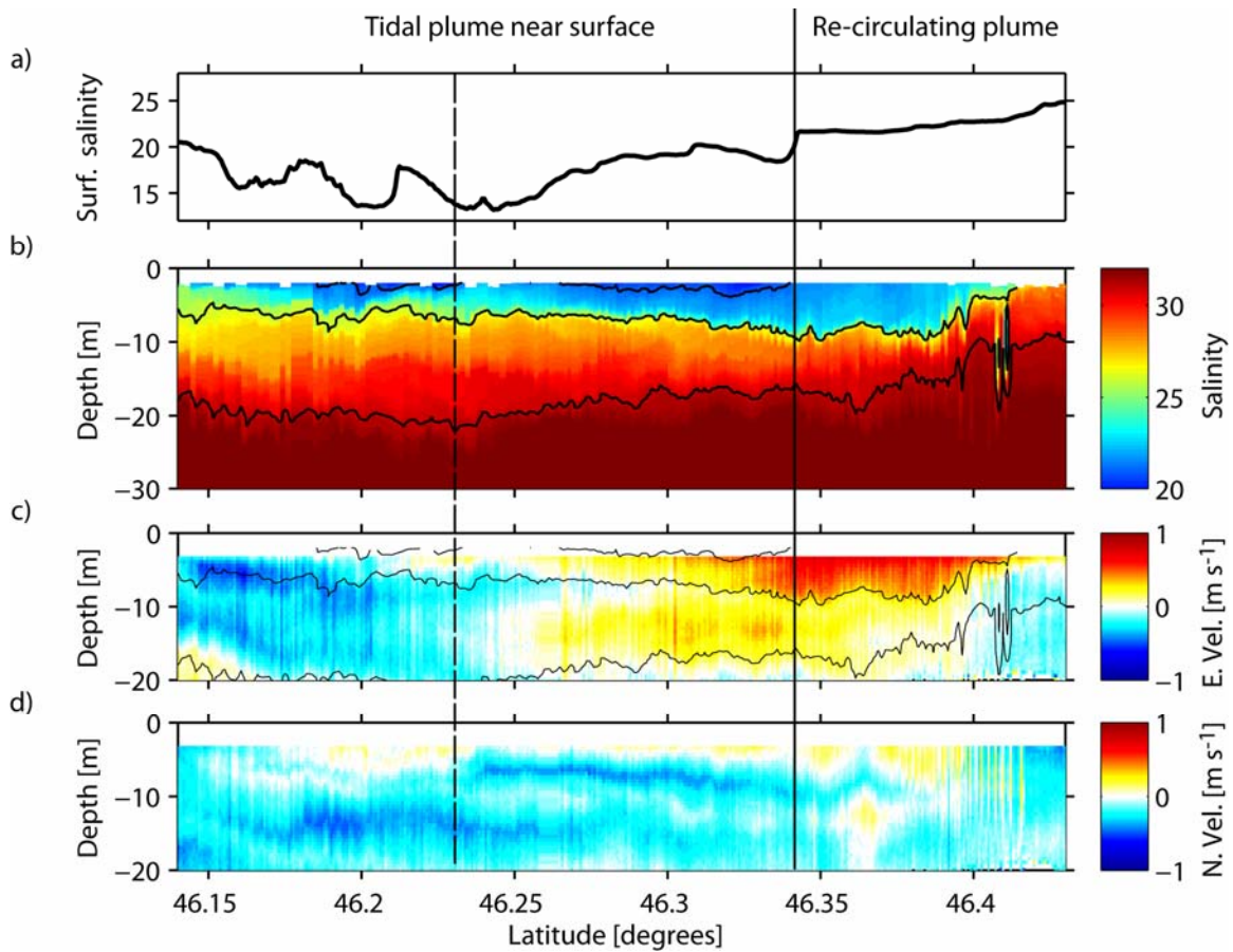
Figure 9: Data from Line B2, 11.6 hours after high tide on June 10, 2005. This transect intersects the anticyclonic circulation in the middle of the plume. a) Surface salinity. b) Salinity from the Triaxus towfish in the upper water column. The black contours are 21, 26 and 32 salinity isohalines, which approximately delineate the tidal, re-circulating and far-field plume water masses. c) and d) show East and North velocity, respectively. Salinity contours from b) are plotted on c) for comparison. The anticyclonic circulation is evident in the East velocity field and the northward flow of the tidal plume can be seen close to the surface in the North velocity field. Solitons, which have been spawned from the tidal plume front are evident in panels b), c) and d) between the front and the northern edge of the re-circulating plume. The vertical solid line marks the northern front of the tidal plume and the dashed line is the approximate axis of the estuary outflow.
