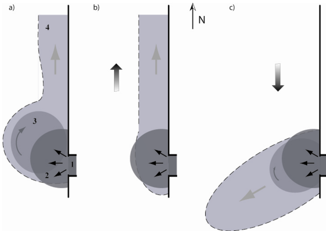
Figure 3: Conceptual model of the Columbia River plume under three wind forcing conditions. a) Plume with low wind forcing showing four water masses: source (1), tidal (2), re-circulating (3) and far-field (4). b) Plume during a period of sustained downwelling wind, which compresses the re-circulating and far-field plumes against the coast resulting in a tidal plume that extends further offshore than the rest of the plume. c) Plume during a period of sustained upwelling wind. In this case the near-surface Ekman flux draws the re-circulating and far-field plumes offshore and the tidal plume propagates primarily into stratified plume water.
