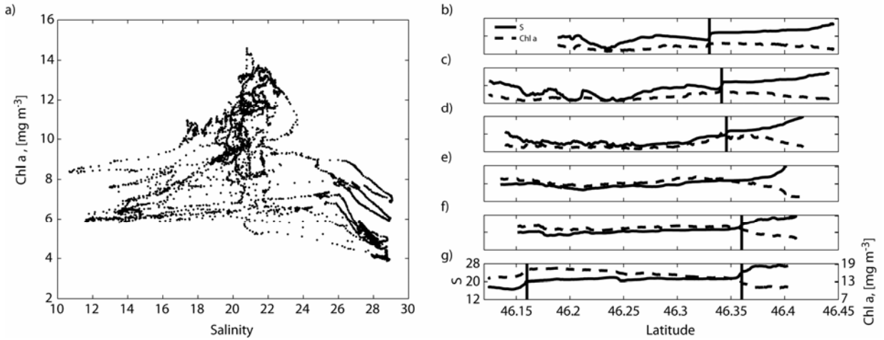
Figure 15: a) Surface chlorophyll a concentration vs. surface salinity for all transects on Line A. High salinity water (far-field plume) is associated with the lowest chlorophyll concentrations, low salinity water (tidal plume) is associated with slightly higher concentrations and intermediate salinity water (re-circulating plume) has the highest chlorophyll concentration. b – g) Surface salinity and chlorophyll a concentration from all transects on Line B.
