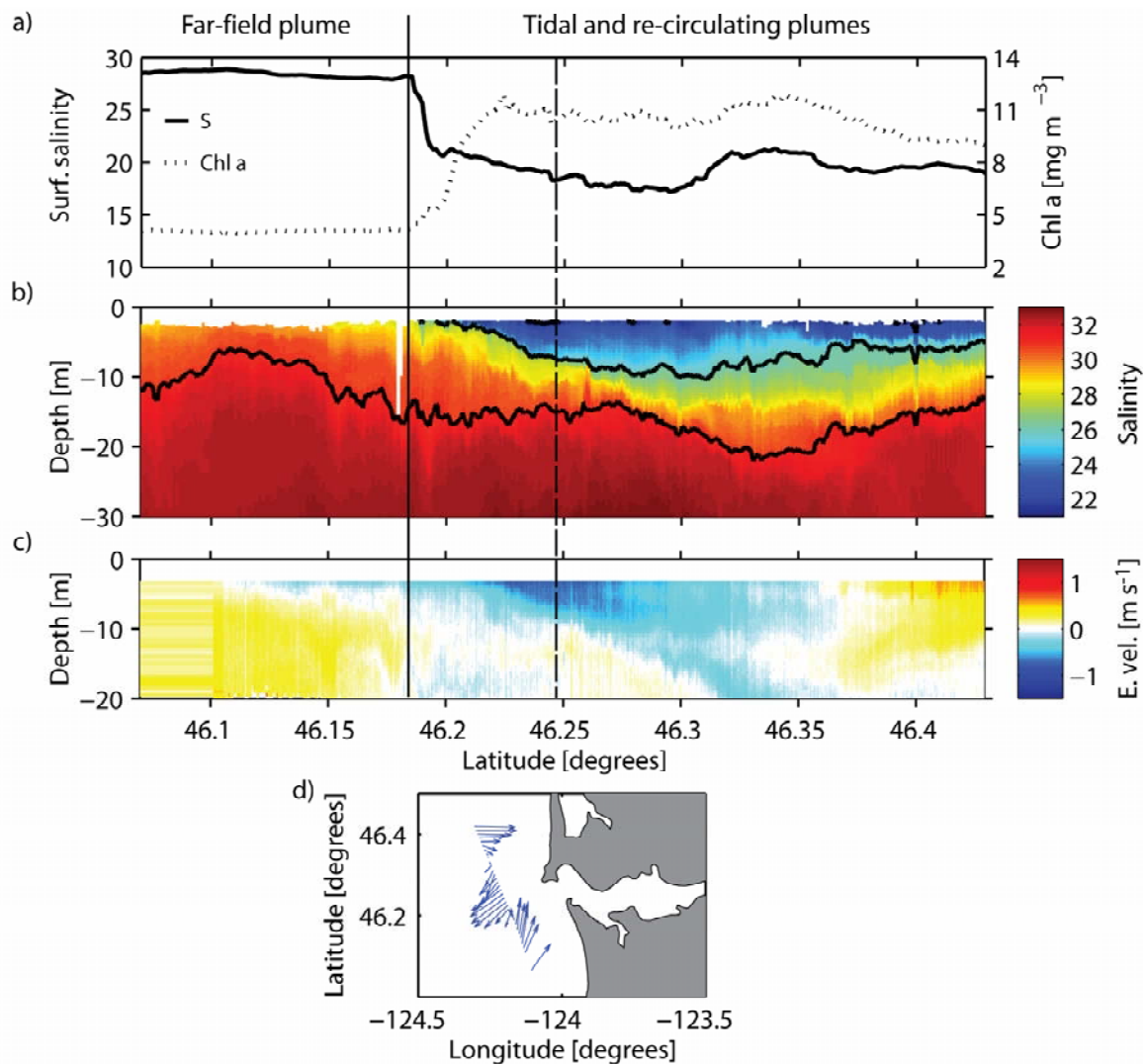
Figure 7: Data from Line A7, 7.1 hours after high tide on June 8, 2005. This transect intersects estuary outflow and clearly shows the anticyclonic circulation. a) Surface salinity (solid) and chlorophyll a concentration (dot) from the vessel underway sampling system. b) Salinity from the Triaxus towfish in the upper water column. The shape of the re-circulating plume is evident in the salinity data, extending from 46.18 to beyond 46.4 degrees North. The black contours are 21, 26 and 32 salinity isohalines, which approximately delineate the tidal, re-circulating and far-field plume water masses. c) East velocity, showing the anticyclonic velocity structure of the re-circulating plume. d) Surface velocity vectors. The solid vertical lines approximately delineate the three offshore water masses according to the surface salinity record. The dashed vertical line marks the approximate axis of the average plume outflow.
