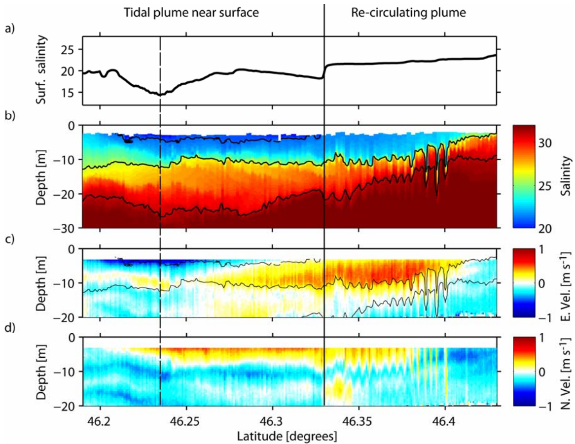
Figure 8: Data from Line B1, 8.9 hours after high tide on June 10, 2005. This transect intersects the anticyclonic circulation in the middle of the plume. a) Surface salinity indicates the location of the northern front of the tidal plume, but shows only a gradual increase toward the northern edge of the re-circulating plume. b) Salinity from the Triaxus towfish in the upper water column. The black contours are 21, 26 and 32 salinity isohalines, which approximately delineate the tidal, re-circulating and far-field plume water masses. c) and d) show East and North velocity, respectively. Salinity contours from b) are plotted on c) for comparison. The anticyclonic circulation is evident in the East velocity field and the northward flow of the tidal plume can be seen close to the surface in the North velocity field. Solitons, which have been spawned from the tidal plume front are evident in panels b), c) and d) between the front and the northern edge of the re-circulating plume. The vertical solid line marks the northern front of the tidal plume, which divides the tidal and re-circulating plumes on the surface. The vertical dashed line marks the approximate axis of the estuary outflow.
