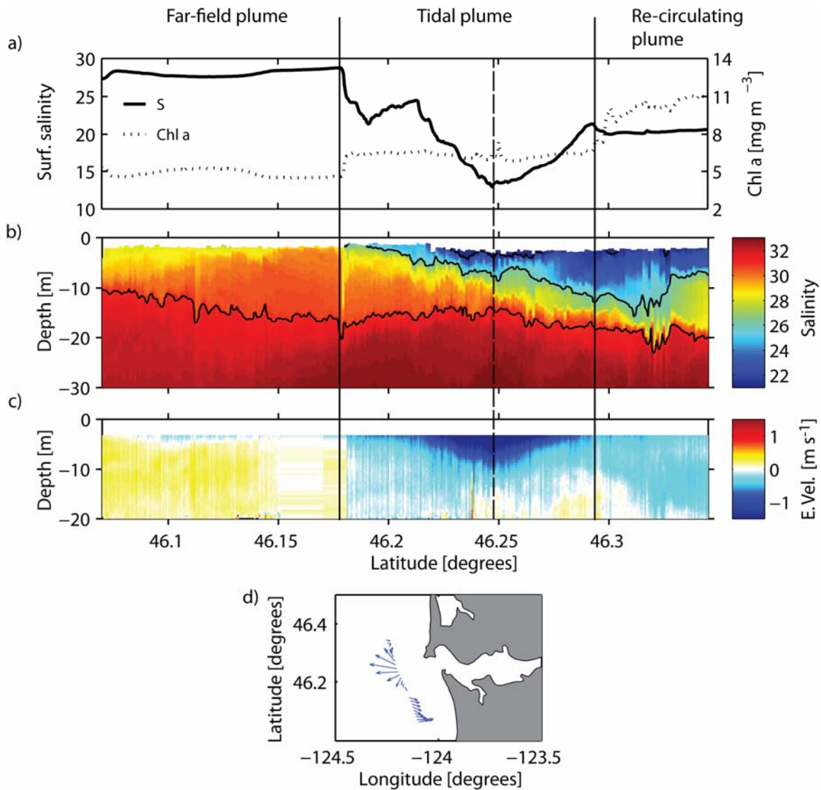
Figure 6: Data from Line A5, 4.2 hours after high tide on June 8, 2005. This transect intersects estuary outflow and the anticyclonic circulation, though the transect was cut short on this pass and the recirculation is not visible. a) Surface salinity (solid) and chlorophyll concentration (dot) from the vessel underway sampling system. b) Salinity from the Triaxus towfish in the upper water column. The black contours are 21, 26 and 32 salinity isohalines, which approximately delineate the tidal, re-circulating and far-field plume water masses. c) East velocity. d) Surface velocity vectors showing the strong, diverging estuary outflow. The solid vertical lines approximately delineate the three offshore water masses according to the surface salinity record. The dashed vertical line marks the approximate axis of the plume outflow.
