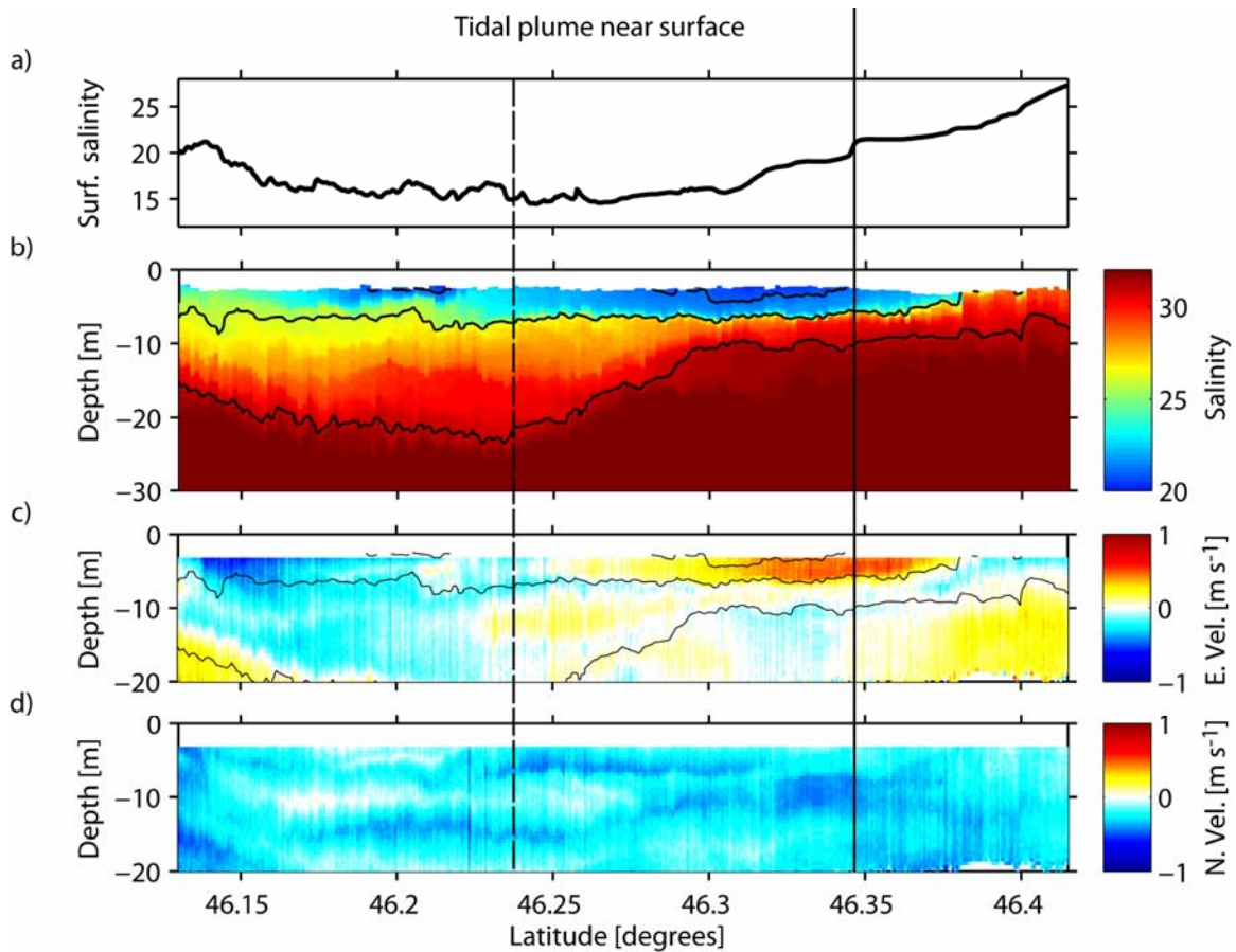
Figure 10: Data from Line B3, 14.7 hours after high tide on June 10, 2005. a) Surface salinity. b) Salinity from the Triaxus towfish in the upper water column. The black contours are 21, 26 and 32 salinity isohalines, which approximately delineate the tidal, re-circulating and far-field plume water masses. c) and d) show East and North velocity, respectively. Salinity contours from b) are plotted on c) for comparison. The anticyclonic velocity structure of the re-circulating plume persists, but the velocity structure associated with the tidal plume has nearly disappeared. The vertical solid line marks the northern front of the tidal plume and the dashed line is the approximate axis of the estuary outflow.
