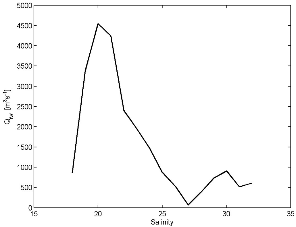
Figure 5: Distribution of freshwater during the ebb tide on June 8, 2005 based on sampling on Line A. The flux was computed assuming a reference salinity of 27 for the coastal waters near the river mouth.
