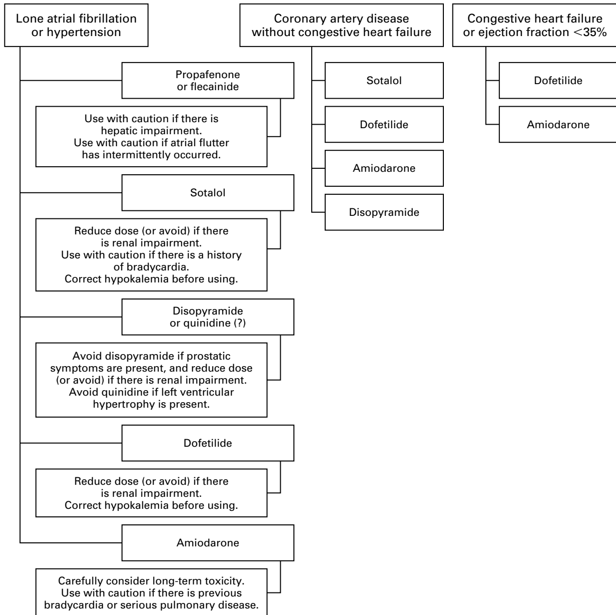
Figure 2. A Suggested Approach for the Selection of Antiarrhythmic Therapy to Maintain Sinus Rhythm after Cardioversion. The order of the listed drugs is merely a guideline. Which drug to use first in each group will depend, to some extent, on the preference of the physician as well as the clinical characteristics of the specific patient. In patients with coronary disease, especially active ischemia, it is prudent to avoid the class IC agents flecainide and propafenone, even though propafenone was not evaluated in the Cardiac Arrhythmia Suppression Trial. Quinidine is included in this figure despite concern about increased mortality with its use, since it is still used widely in some countries and no comparative mortality studies have been performed.
