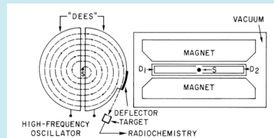
Fig. 7-2. Schematic representation of a cyclotron; top (left) and side (right) views. D1 and D2 are the "dees" to which the accelerating voltage is applied by a high-frequency oscillator. Target line may feed directly to a radiochemistry area.
