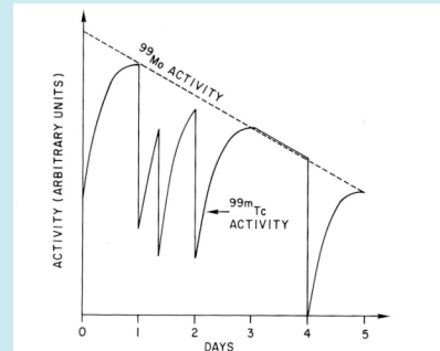
Fig. 7-6. Buildup and decay of ^{99m}\text{Tc} generator eluted on days 0, 1, 1.4, 2, and 4.
