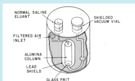
Fig. 7-5. Cross-sectional drawing of a ^{99}\text{Mo} - ^{99\text{m}}\text{Tc} generator. (Courtesy of the Society of Nuclear Medicine and Thomas R. Goss.)
