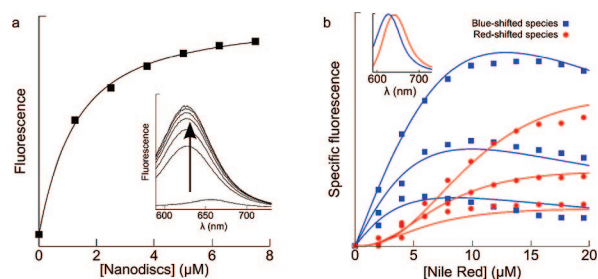
Figure 1. (a) NR (0.5 \mu\text{M} ; \lambda_{\text{ex}} = 550 \text{ nm} ) fluorescence increasing with [Nanodiscs] yields a K_D of 1 \mu\text{M} for a singly occupied disk. (b) NR fluorescence increases and red-shifts with increasing [NR], at three different Nanodisc concentrations, 0.5, 1.0, and 2.0 \mu\text{M} . Solid lines are global fits with five sequential NR binding modes and a negative cooperativity factor of 2.3. (Inset) Basis spectra used in singular value decomposition to deconvolute the spectral shift.
