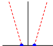
(f) vapnik, \varepsilon = 0.5
