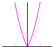
(i) elastic net, \alpha = 0.5
