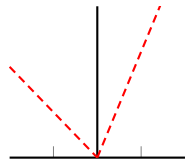
(c) quantile, \tau = 0.3
