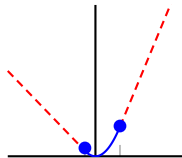
(e) quantile huber
