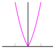
(i) elastic net, \alpha = 0.5
