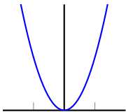
(a) quadratic
