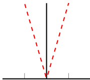
(b) 1-norm
