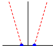
(f) vapnik, \epsilon = 0.5
