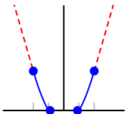
(g) huber ins. loss
