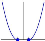
(h) quadratic ins. loss
