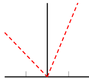
(c) quantile, \tau = 0.3
