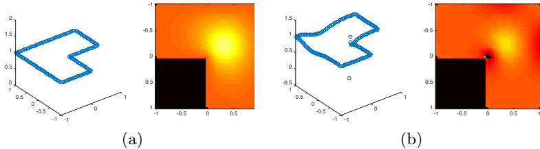
Fig. 3.2: Boundary values, u , and solution in the interior for the initial and optimized boundary values are depicted in (a) and (b) respectively.
