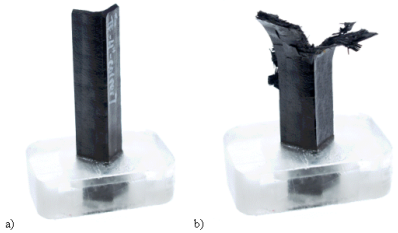
Figure 10 a, b. Small corner element, specimen IV, before and after crush testing
