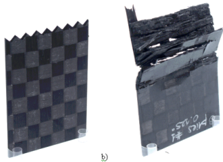
Figure 19 a, b. Flat specimen, before crushing showing the saw-tooth trigger (a), and after crushing (b) at 12.5 mm of unsupported height.
