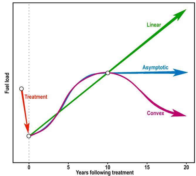
Fig. 6. Hypothetical demonstration of the limitations of infrequent re-measurement, with three possible trajectories of fuel profile and stand structure responses to treatment over time. The horizontal axis shows time since treatment, with the dotted vertical line representing the time of treatment implementation. The vertical axis represents the quantity of a fuel component of interest. The open circles identify three re-measurements as in a typical data collection schedule for treatment longevity studies. Note that it is impossible to distinguish trajectories from these limited data, and that the asymptotic and convex trajectories diverge after the last measurement. Pre-treatment sample period is presented to illustrate common study designs.
