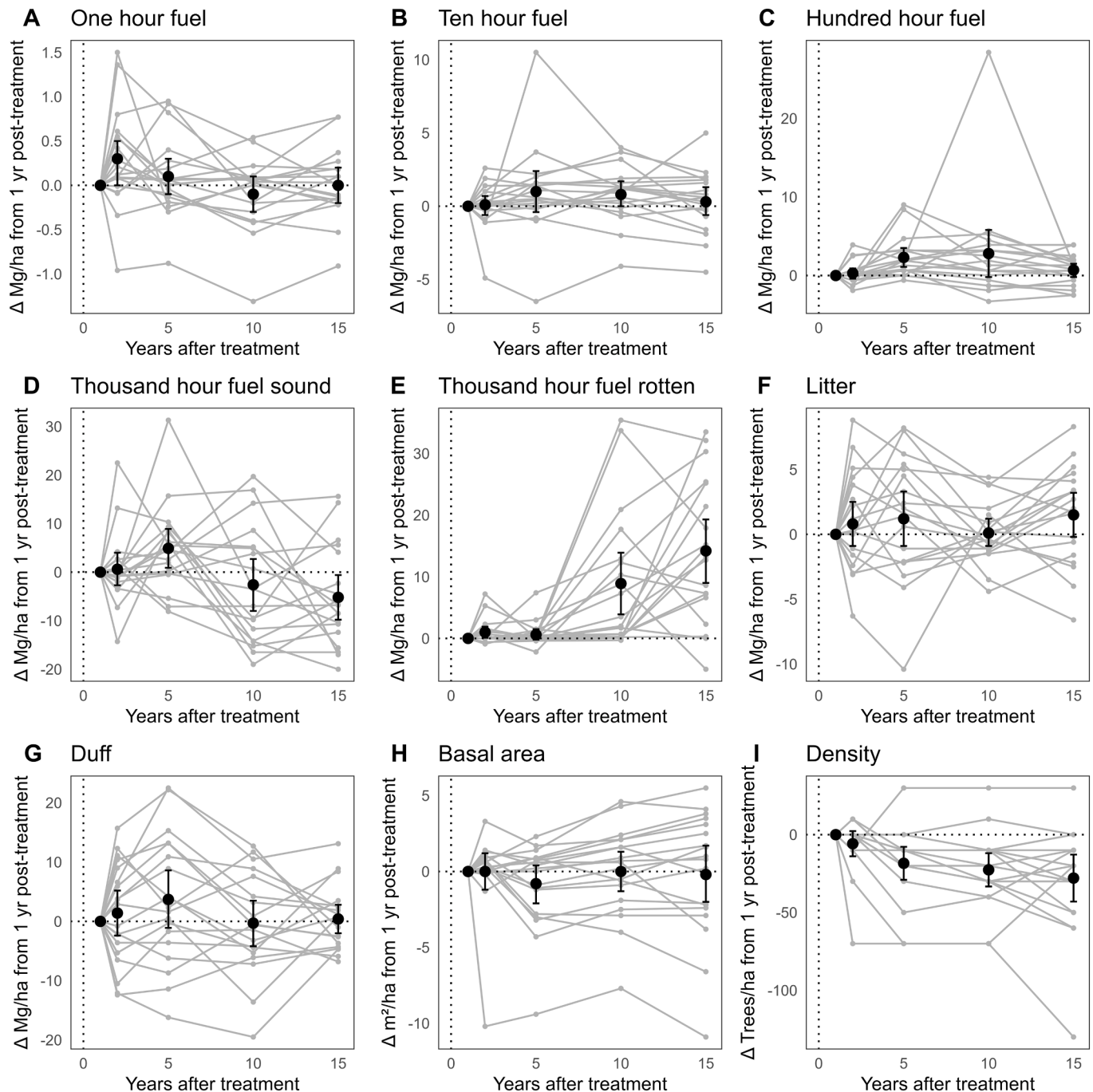
Fig. 5. Fuel profile and stand structure trajectories over time showing variable and nonlinear responses with time since treatment. Data are from 19 permanent plots sampled repeatedly at identical intervals after thin-plus-burn treatments (Radcliffe, 2024). The values at each sample period are expressed relative to short-term treatment values (1 year following treatment). Black dots represent means within time periods, black bars represent 95 % confidence intervals around those means. Gray lines show the trajectories of individual plots; lines connect measurements but are not intended to imply linear changes between sample periods. Vertical dotted lines represent the time of burn implementation in the “thin-plus-burn” sequence. Data are from the National Park Service Fire Effects Monitoring Program at the North Cascades and Lake Roosevelt National Recreation Areas of Washington state (USDI National Park Service, 2003).
