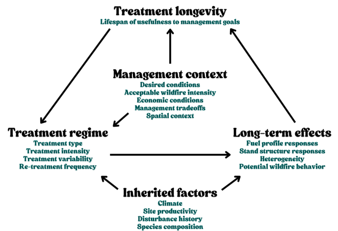
Fig. 3. Treatment longevity is determined by the interaction between management context and long-term treatment effects.
