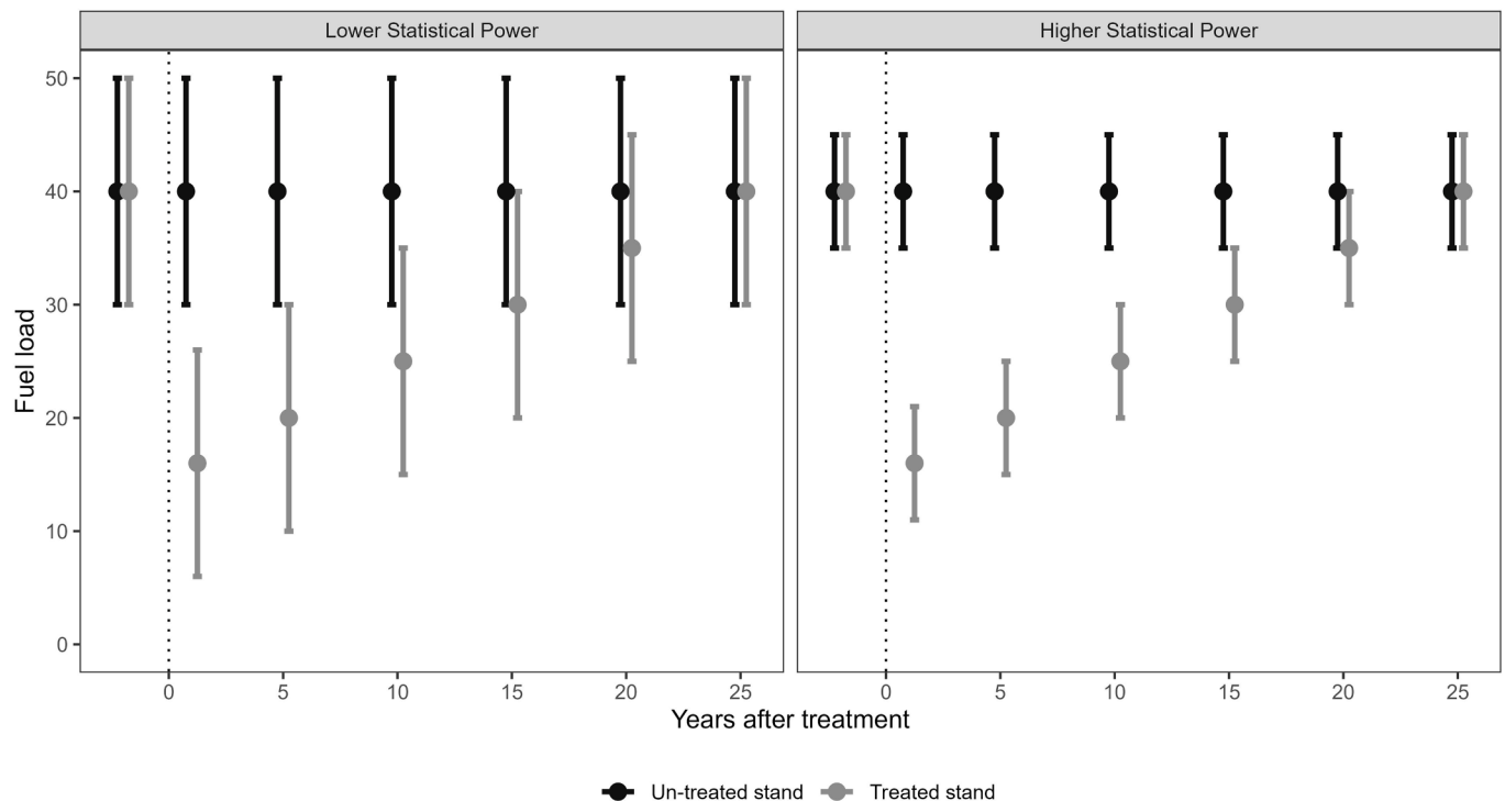
Fig. 4. Hypothetical demonstration of statistical power's influence on estimating treatment longevity. Left and right panels differ only in the level of statistical uncertainty in mean fuel loads over time. Dots represent mean fuel loads, lines bounded by ticks represent confidence intervals reflecting a researcher-chosen alpha level. If treatment longevity were determined by statistical significance, and the confidence interval overlap is used as determinant of statistical significance, a treatment would be effective for 5 years in the lower statistical power scenario and for 15 years in the higher statistical power scenario. Simplifying assumptions in this example include a static fuel load in the un-treated stands, linear increase of fuel loads with time since treatment in the treated stands, and identical statistical power for the un-treated and treated stands.
