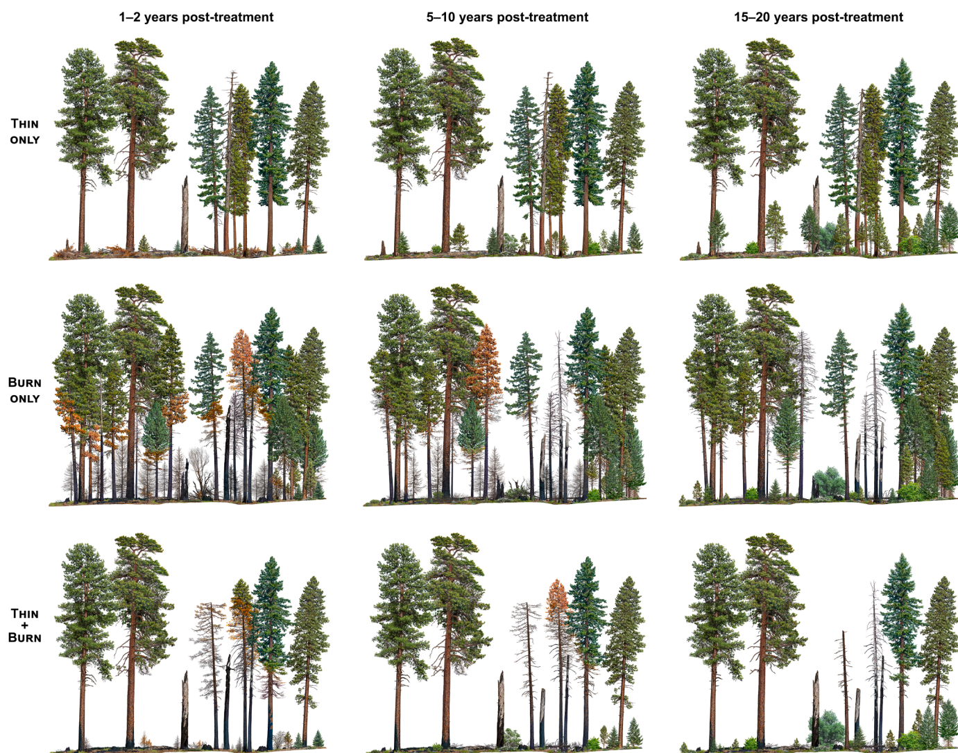
Fig. 2. Conceptual long-term treatment effects in the stand displayed in Fig. 1, following application of three common treatment types. This representation is a heuristic starting point for understanding long-term treatment effects; outcomes of specific treatments will vary. The thin-only treatment represents a thin from below without follow-up slash management. The burn-only treatment represents a prescribed low intensity broadcast burn. The thin-plus-burn treatment represents a thin from below followed one year later by a prescribed broadcast burn of relatively low intensity. Note fine-scale variation in treatment intensity and long-term responses following treatment. See Appendix 1 for more detailed views and explanations of individual panels. Paintings by Robert Van Pelt.
