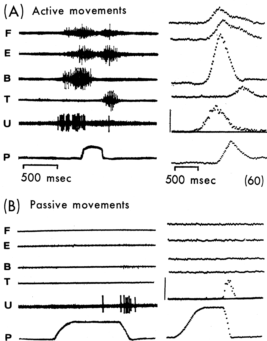
Fig. 2. Responses of precentral cell and arm muscles during active and passive elbow movements. Successive lines from top to bottom show activity of flexor carpi radialis ( F ), extensor carpi radialis ( E ), biceps ( B ), triceps ( T ), cortical unit ( U ), and the position of the elbow ( P ). A single trial is shown at left, and the averages over 60 successive trials at right. This cell fired before active flexion of the elbow ( A ) and responded to passive extension of the elbow ( B ). All EMG averages were computed at identical gains. Time histogram of cell activity is shown with a zero baseline; vertical calibration bar equals 50 impulses per second. Upward deflection of the position monitor represents flexion.
