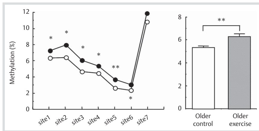
Fig. 3 Methylation of ASC and exercise in older groups. Left: Methylation rates of all 7 targeted sites. Open circles: older control group (n=153). Closed circles: older exercise group (n=230), after 6-month interval walking regimen. Right: Difference in mean methylation values of the 7 sites between the older control group and the older exercise group. Values are written as mean \pm SE. * p < 0.05 , ** p < 0.01
