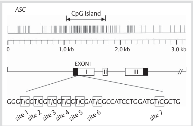
Fig. 1 Schematic view of the ASC gene region analyzed in this study. Seven CpG sites in the CpG island were designated for pyrosequencing analysis based on the effective region from Conway et al. [5].
