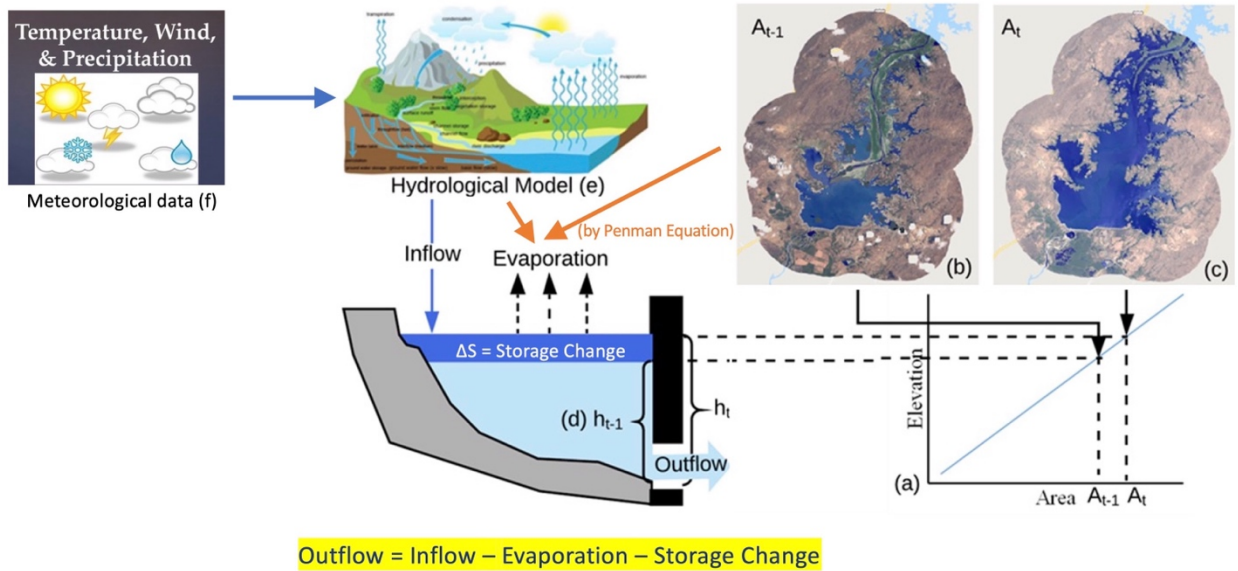
650 Figure 2: Conceptual model of RAT and the mass balance equation.
