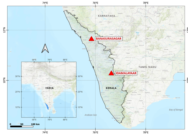
Figure 12: Map of Kerala with the location of the Banasurashagar and Idamalayaar dam. After Suresh et al. (2023)
