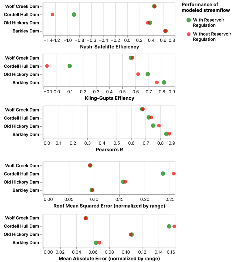
Figure 14: Performance of RAT-generated regulated inflow using ResORR compared to the unregulated inflow modeled using VIC in the regulated Cumberland River basin in terms of performance metrics. The chart shows that it is clearly improving simulations when compared to the baseline (unregulated inflow) for most dams.
