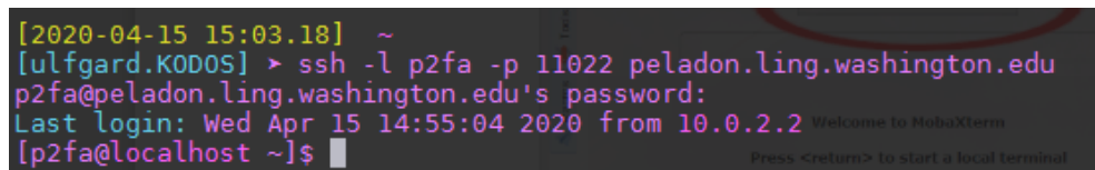
Figure 2: Logging into a remote host
