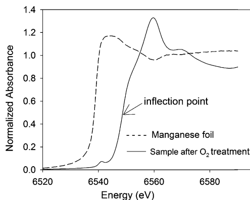
Figure 9. XANES spectra characterizing the sample prepared from Mn 2 (CO) 10 on MgO (1.0 wt % Mn) after O 2 treatment and manganese foil.
