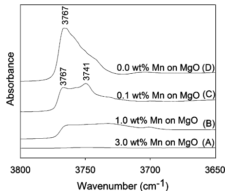
Figure 2. Normalized IR spectra in the \nu_{OH} region characterizing sample prepared from Mn_2(CO)_{10} on MgO. The respective Mn contents (wt %) of the samples were 3.0 (A), 1.0 (B), 0.10 (C), and 0.0 (D). Spectra were normalized with respect to the carbonate band at 1264 \text{ cm}^{-1} .
