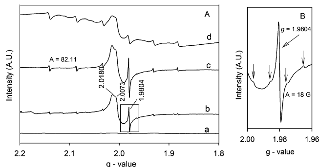
Figure 1. (A) EPR spectra of untreated MgO (a), MgO after treatment in O_2 at 673 K followed by evacuation at the same temperature (b), sample prepared from Mn_2(CO)_{10} on MgO (0.10 wt % Mn) (c), and sample prepared from Mn_2(CO)_{10} on MgO (1.0 wt % Mn) (d); (B) magnification of part A, spectrum b, at g \approx 1.9804 .
