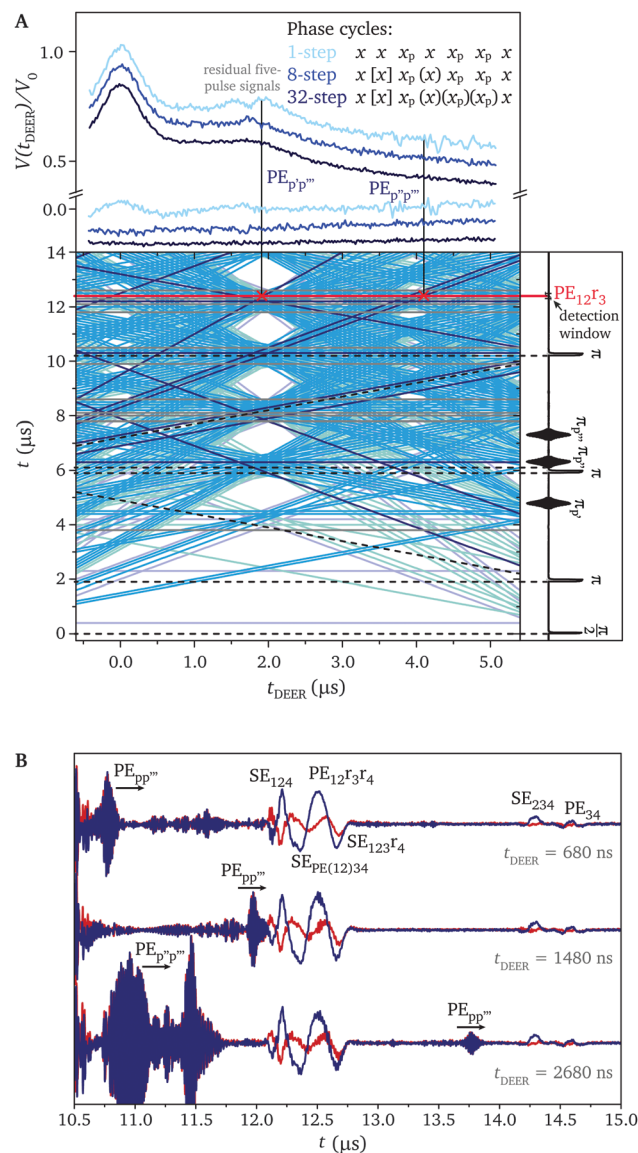
Fig. 9 (A) Positions of the echo crossings in a seven-pulse DEER experiment with the following inter-pulse delays \tau_1 = 1.9 \mu\text{s} , \tau_2 = 2.1 \mu\text{s} and t_2 = 200 \text{ ns} . The pulse sequence is plotted along the y-axis with pulse positions represented by dashed lines. The standing echoes of the observer sequence are shown in grey and the different types of echoes induced by the pump pulses are shown in different shades of blue following the same colour code as in Fig. 3. Seven-pulse DEER traces recorded with different phase cycles are shown in the top panel. The traces are offset to allow better comparison. The crossing positions of the two strongest moving echoes with the detected refocused echo ( PE_{12}r_3 , position shown in red) are highlighted and tentatively assigned. (B) Echo transients recorded at three points in the DEER experiment. The echoes that could be assigned are labelled following the conventions used for the four- and five-pulse experiments and the direction of movement for crossing echoes is indicated by arrows.
