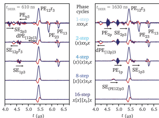
Fig. 7 Echo transients recorded for two different positions of a monochromatic rectangular pump pulse ( t_{DEER} = 610 ns (left) and t_{DEER} = 1630 ns (right)) for different phase cycles of the four-pulse DEER experiment. The experimental parameters are the same as reported in Fig. 6. The different echoes are labelled according to the notation of Table 1 and the arrows indicate their direction of movement.
