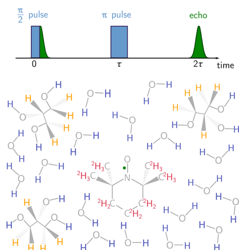
Figure 1. (top) Measuring the Hahn echo amplitude as a function of total pulse sequence length, 2\tau , provides the simplest way to observe decoherence effects. (bottom) The system under study is d_{18} -TEMPO (unpaired electron shown in green) solvated in a frozen 1:1 mass:mass ( \approx 5:1 mol:mol) water:glycerol solution, with solvent exchangeable hydrons (blue), solvent nonexchangeable hydrons (yellow), and TEMPO's deuterons (red) contributing to decoherence.
