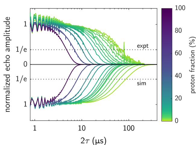
Figure 2. Experimental Hahn echo decays (upper part; 20 K, 1.2 T, 33.8 GHz) and simulated decays (lower part; reflected) are shown as a function of proton fraction (color-coded) for 5 \mu\text{M} d_{18} -TEMPO in a 1:1 water:glycerol matrix where the proton concentration was varied between natural abundance and 1 M via the ratio of \text{H}_2\text{O} : h_8 -glycerol to \text{D}_2\text{O} : d_8 -glycerol.
