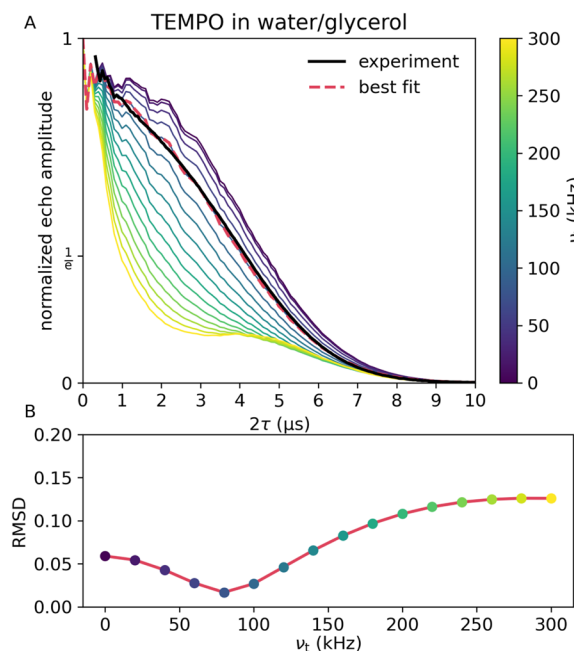
FIG. 4. Panel (a) plots the 20 K experimental (black) and simulated Hahn echo decays of TEMPO in frozen 1:1 mass:mass water:glycerol solution. The color axis indicates the value of the tunnel splitting used for the TEMPO methyls in the simulations. Cutoffs: 10^{-7} (rad/μs) 4 for k\omega^4 and 323 \times 10^{-7} for k . The experimental data are scaled to minimize their RMSD with the 80 kHz tunnel splitting simulation. Panel (b) shows the RMSD of each simulation with the experimental data. In evaluating the RMSD at each tunnel splitting, the scaling of the experimental data was set to minimize the RMSD.
