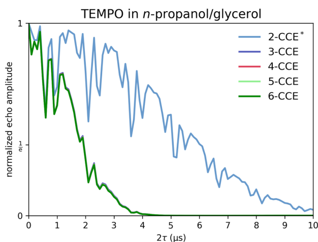
FIG. 5. This figure shows CCE simulations of the Hahn echo decay of TEMPO in n -propanol/glycerol at a single orientation, using cutoffs of 10^{-7} \text{ (rad/}\mu\text{s)}^4 and 323 \times 10^{-7} for k\omega^4 and k , respectively, and tunnel splittings of 80 kHz for both nitroxide and n -propanol methyls. (*) It should be noted that since partial methyls are not included, neither methyl tunneling effects nor methyl proton flip-flops are included in 2-CCE.
