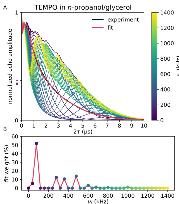
FIG. 6. Panel (a) shows the experimental and 4-CCE simulated Hahn echo decays of TEMPO in 1:3 volume:volume n -propanol:glycerol solution plotted vs 2\tau . The black trace represents the experimental data, acquired at 20 K. The simulations use 80 kHz tunnel splitting for the four TEMPO methyl groups, and varied the n -propanol methyl tunnel splitting 0–1400 kHz, indicated by the color-axis. Cutoffs: 10^{-7} \text{ (rad/}\mu\text{s)}^4 for k\omega^4 and 323 \times 10^{-7} for k . The red curve represents a linear combination of the simulations from a non-negative least squares fit to the experimental data. The fit and the experimental data are scaled so that the fit is unity at 2\tau = 0 . Panel (b) shows the fit weights against the n -propanol methyl tunnel splittings. The fit has \text{RMSD} = 0.09 , and a coefficient of determination is 0.999. The mode n -propanol methyl tunnel splitting is at 80 kHz. The data are colored by their tunnel splitting to make comparisons with the simulated decays easier. The weights are connected by the red line to guide the eye and show the relationship to the fit in panel (a).
