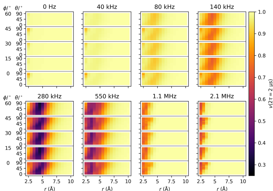
FIG. 9. Echo amplitude v(2\tau = 2 \mu\text{s}) vs r simulated for various tunnel splittings up to 2.1 MHz, are shown as a function of electron–methyl distance ( r ) and relative methyl orientation ( \theta and \phi ), using a H–H distance of 1.78 Å and a magnetic field of 1.2 T.
