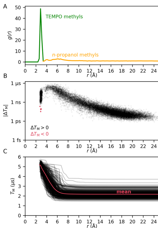
FIG. 7. Panel (a) shows the electron–methyl radial correlation function for TEMPO in n -propanol/glycerol over all MD frames. The distances are from the midpoint of the TEMPO NO bond to the centroid of the methyl protons. The color indicates the dominant nature of the methyl groups at each distance: green for TEMPO and yellow for n -propanol. Panel (b) plots each methyl from each frame as its distance from the detected electron and the change in T_M when its tunnel splitting is turned off: the black points are for \Delta T_M > 0 and indicate that turning the tunnel splitting off lengthens the coherence time, while the red points are for \Delta T_M < 0 for the few cases where turning the tunnel splitting off reduces the phase memory time. Panel (c) plots for each of the 301 MD frames the T_M when only methyls up to distance r of the electron have a non-zero tunnel splitting, 80 kHz for both TEMPO and for n -propanol. In addition, the average T_M(r) is shown in red.
