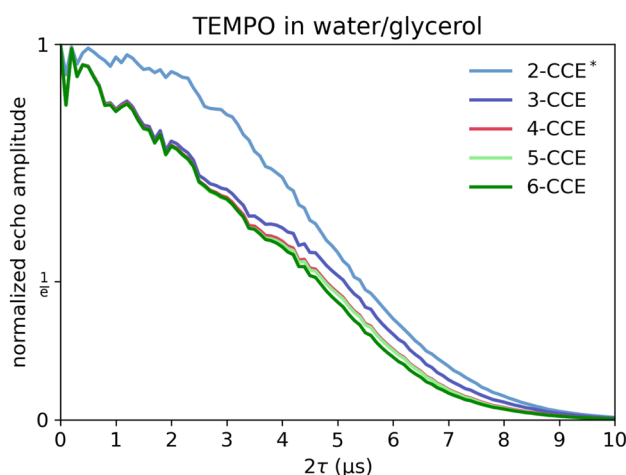
FIG. 3. This figure shows CCE simulations of the Hahn echo decay of TEMPO in 1:1 mass:mass water:glycerol at a single orientation, using cutoffs of 10^{-7} (rad/μs) 4 and 323 \times 10^{-7} for k\omega^4 and k , respectively, and an 80 kHz tunnel splitting for the TEMPO methyls. (*) It should be noted that since partial methyls are not included, neither methyl tunneling effects nor methyl proton flip-flops are included in 2-CCE.
