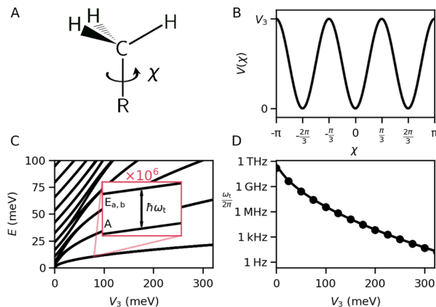
FIG. 1. Structure and energetics of a methyl group: Panel (a) shows a Lewis structure of a methyl group, with the definition of the rotation angle \chi . Panel (b) plots the rotational potential energy function against \chi . Panel (c) shows how rotational energy levels vary with the barrier height, V_3 . While not visible at this scale, the visible energy levels are split into an A state and two degenerate E states, separated by the tunnel splitting for that level. This is shown in the inset at a million times the magnification of the main plot for the ground state at V_3 \approx 80 meV, where \nu_t \approx 18 MHz. Panel (d) shows the tunnel splitting for the ground librational level, as a function of barrier height. The dots indicate values obtained by numerically diagonalizing the rotational Hamiltonian. 38 The solid line shows the approximate analytic expression of Eq. (14). The logarithmic scale of \omega_t/2\pi should be noted.
