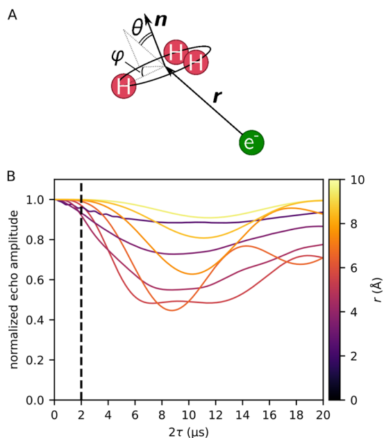
FIG. 8. Panel (a) shows the methyl group at position r relative to the electron; r points toward the methyl proton center of mass. The angle between r and the vector normal to the hydrogen plane, n , is denoted \theta , and the angle between the projection of -r onto the hydrogen plane and the hydrogen anticlockwise of the projection is \phi . Panel (b) shows the calculated orientationally averaged echo modulations for \theta = \phi = 0 and |r| \in \{2.5, 3.5, 4.5, 5.5, 6.5, 7.5, 8.5, 9.5\} Å (indicated on the color axis) and with a 80 kHz methyl torsional tunnel splitting. A dashed line is drawn at 2\tau = 2 \mu\text{s} .
