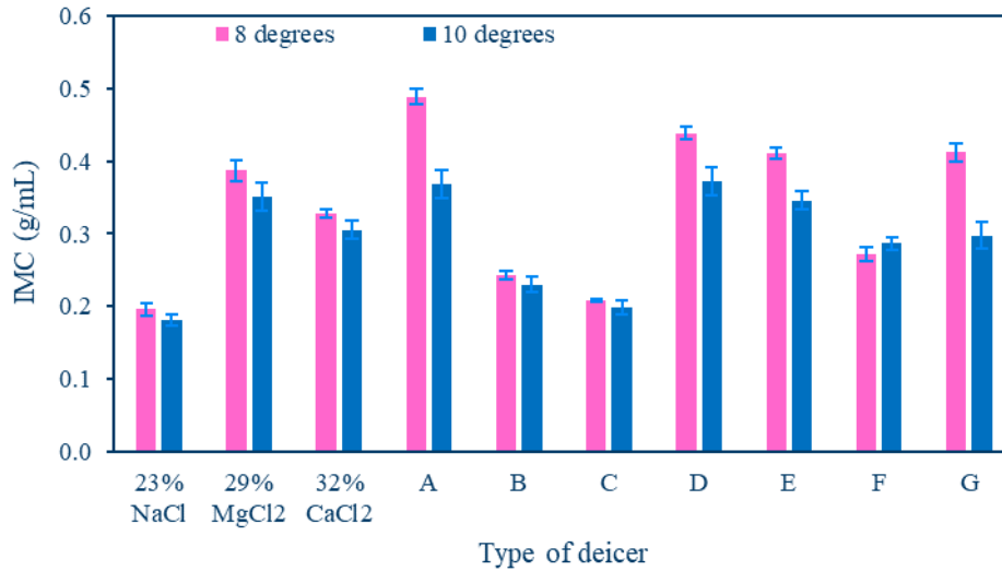
Figure 3-3 IMC results obtained by the WSU teams for different deicers at two different tilt angles of 8° and 10° (error bars indicate ± SD).
