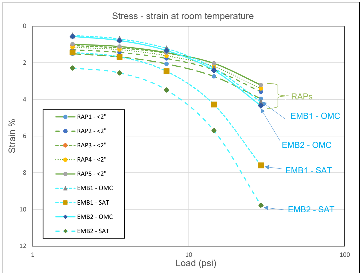
FIGURE 66. Unprocessed RAP (< 2-in. sieve) vs. soil under different load increments at room temperature.
