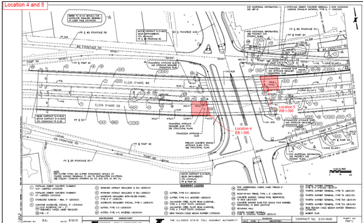
FIGURE 39. Locations 4 and 5 of settlement at Elgin O'Hare Expressway.
