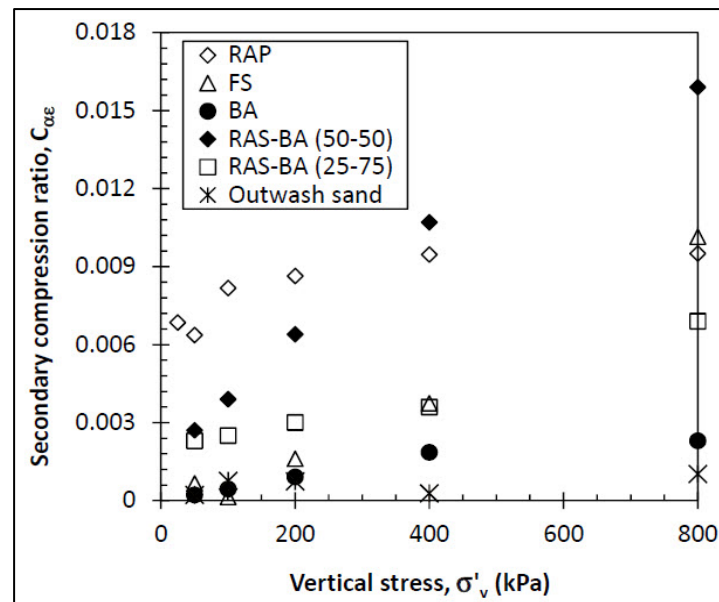
FIGURE 14. Change in secondary compression ratio of different materials with change in vertical stress (FS: foundry slag, BA: bottom ash, RAS: recycled asphalt shingles) (Soleimanbeigi et al., 2014).
