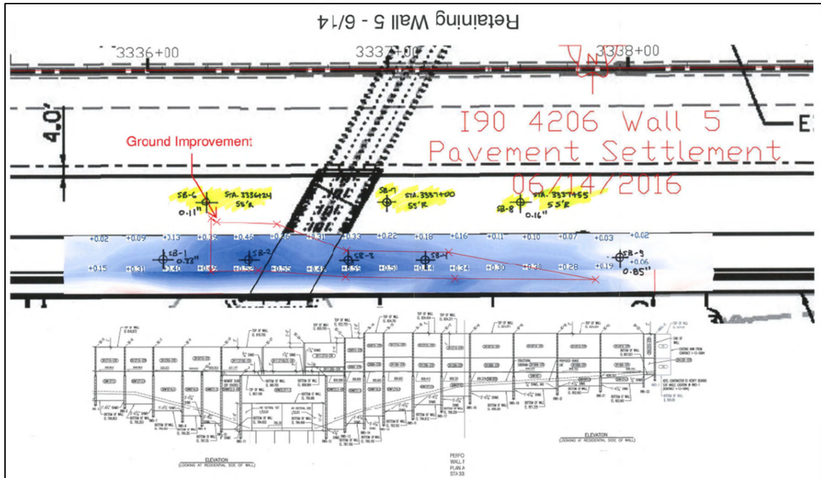
FIGURE 32. Failure locations next to Retaining Wall #5 (Station 3336+00 – Station 3338+00).
