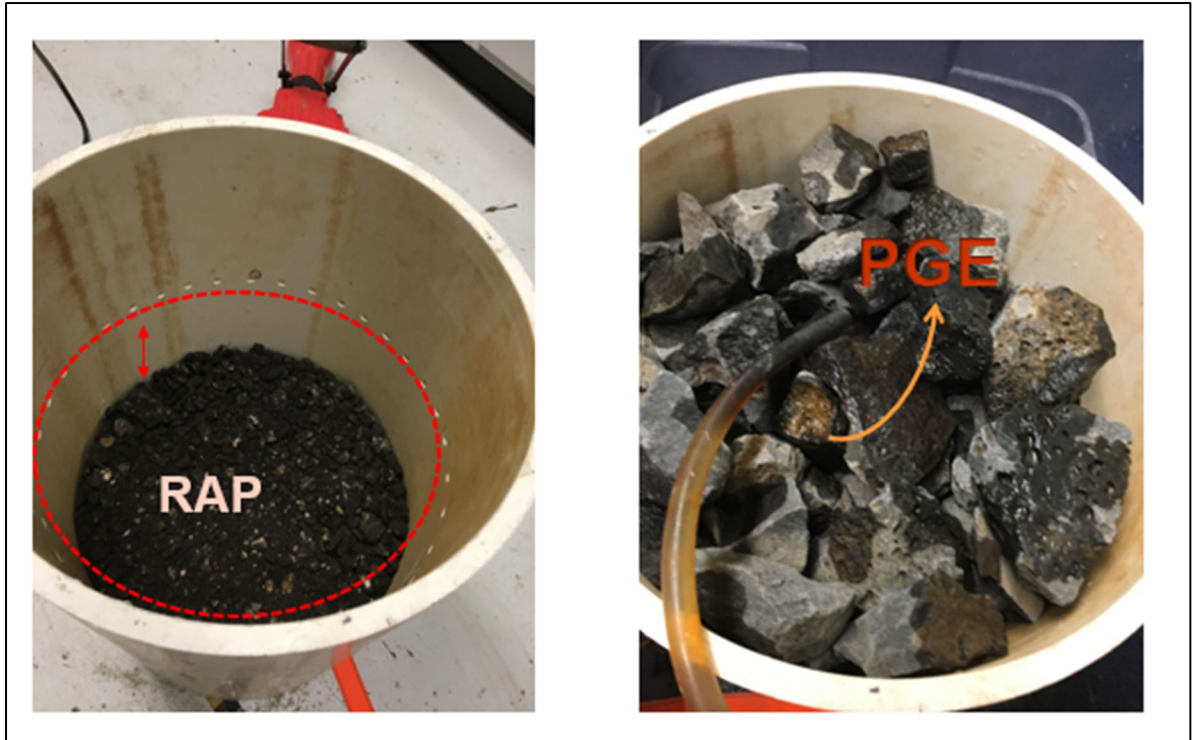
FIGURE 47. RAP and rocks (porous granular embankment, or PGE) in permeability tube.
