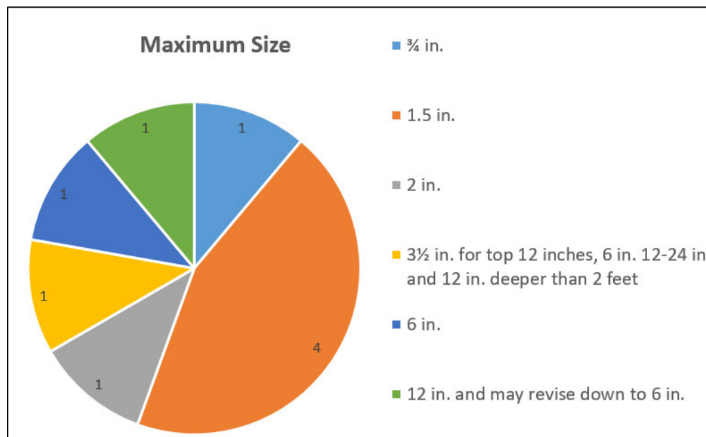
FIGURE 21. Maximum size of RAP particles specified by several state DOTs.
