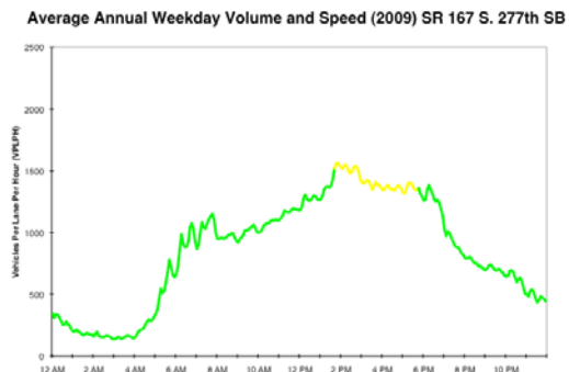
Figure E-3: Example Traffic Volume Pattern with Modest Midday Volume
