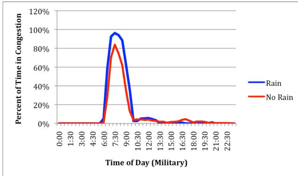
Figure 11: The Probability of Being in Congestion: Rain versus No Rain I-90 Westbound from Issaquah to Bellevue
