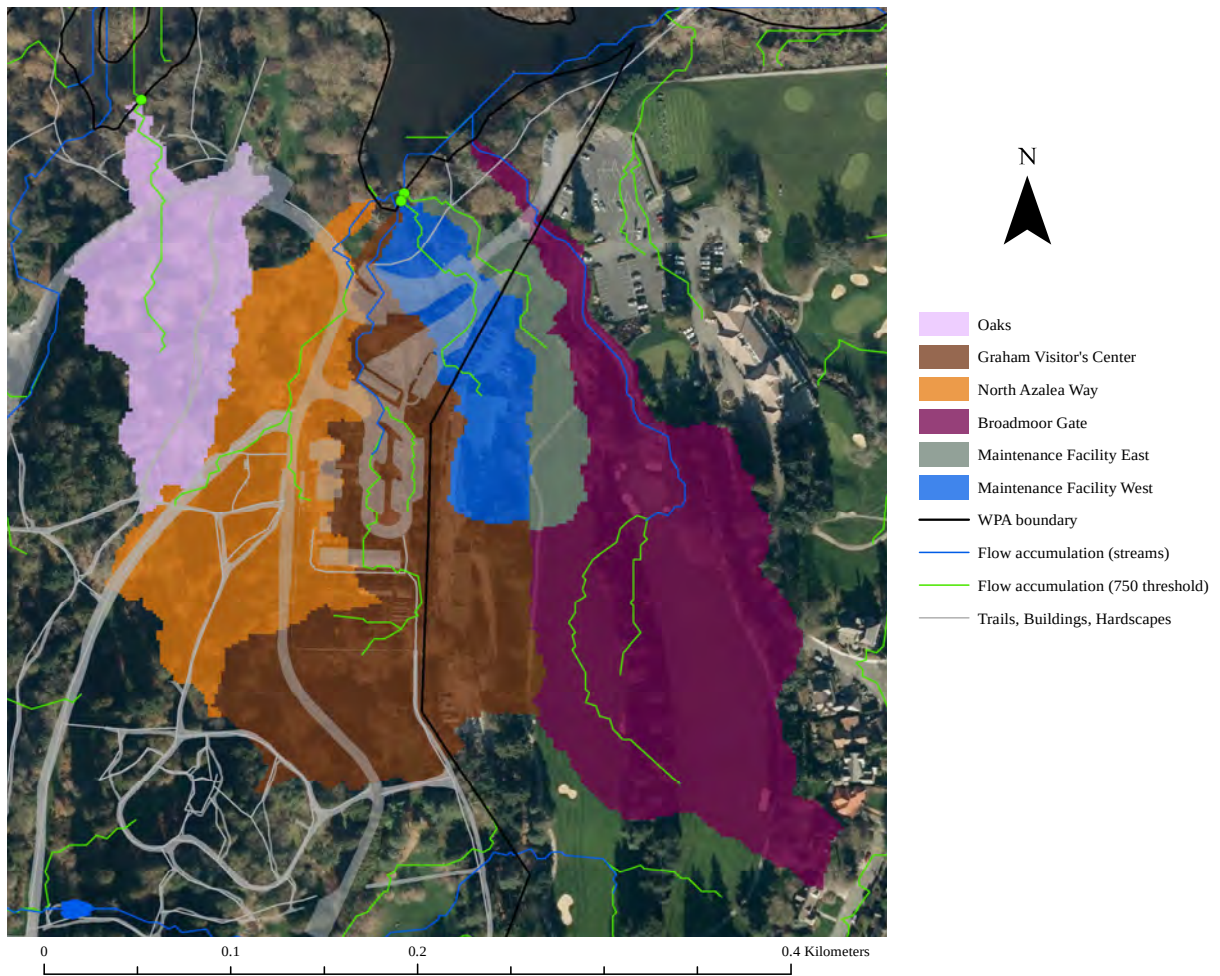
Figure 31. Minor watersheds (Maintenance Facility West, Maintenance Facility East and Oaks watersheds delineated on 750 cell flow accumulation threshold)
