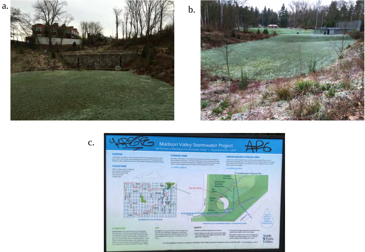
Figure 29. The Madison Valley Stormwater Project completed in 2012 by Seattle Public Utilities: (a) stormwater storage tank, (b) aboveground overflow retention area and (c) interpretative sign
