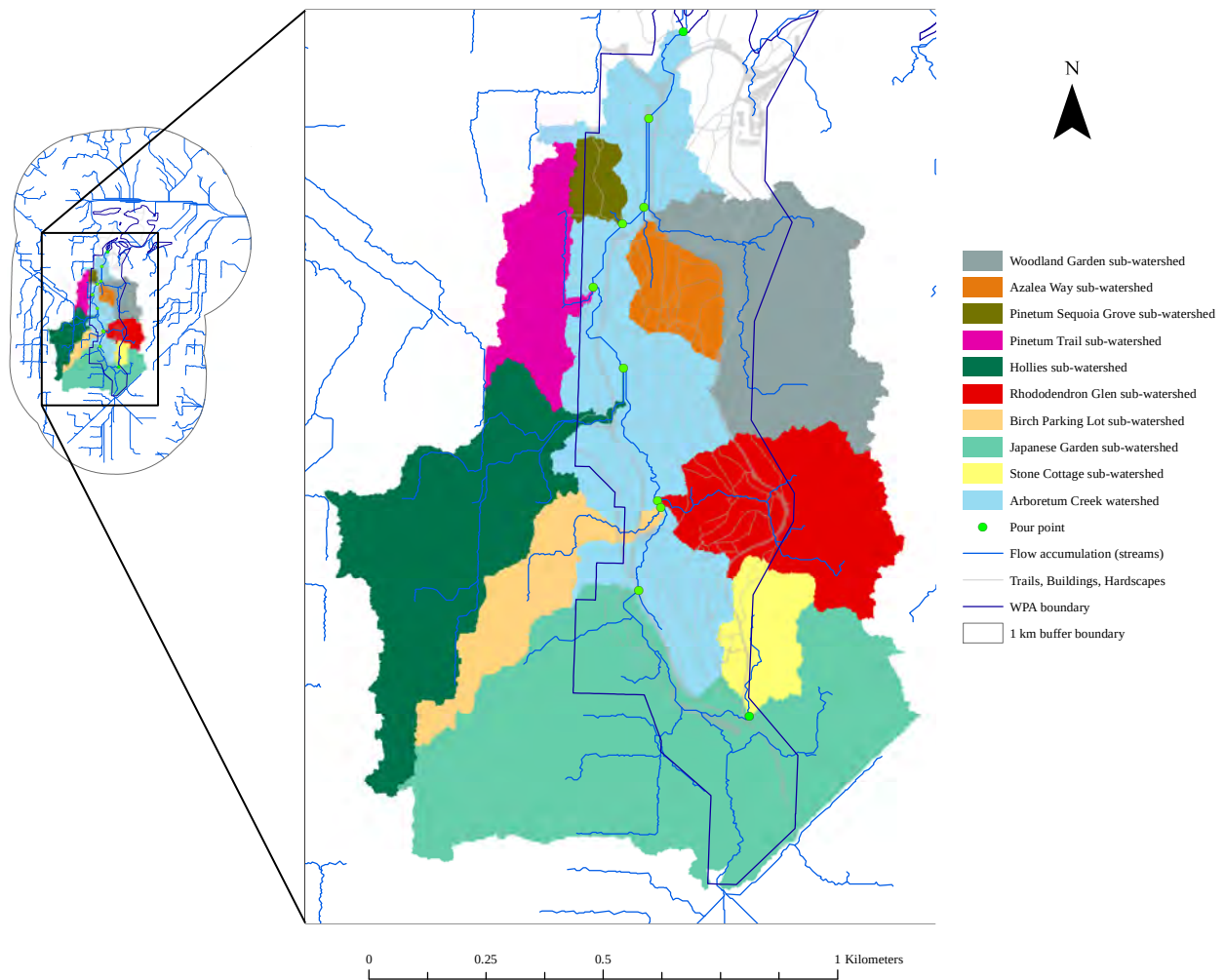
Figure 11. Sub-watersheds of Arboretum Creek (MVSP has been omitted)
